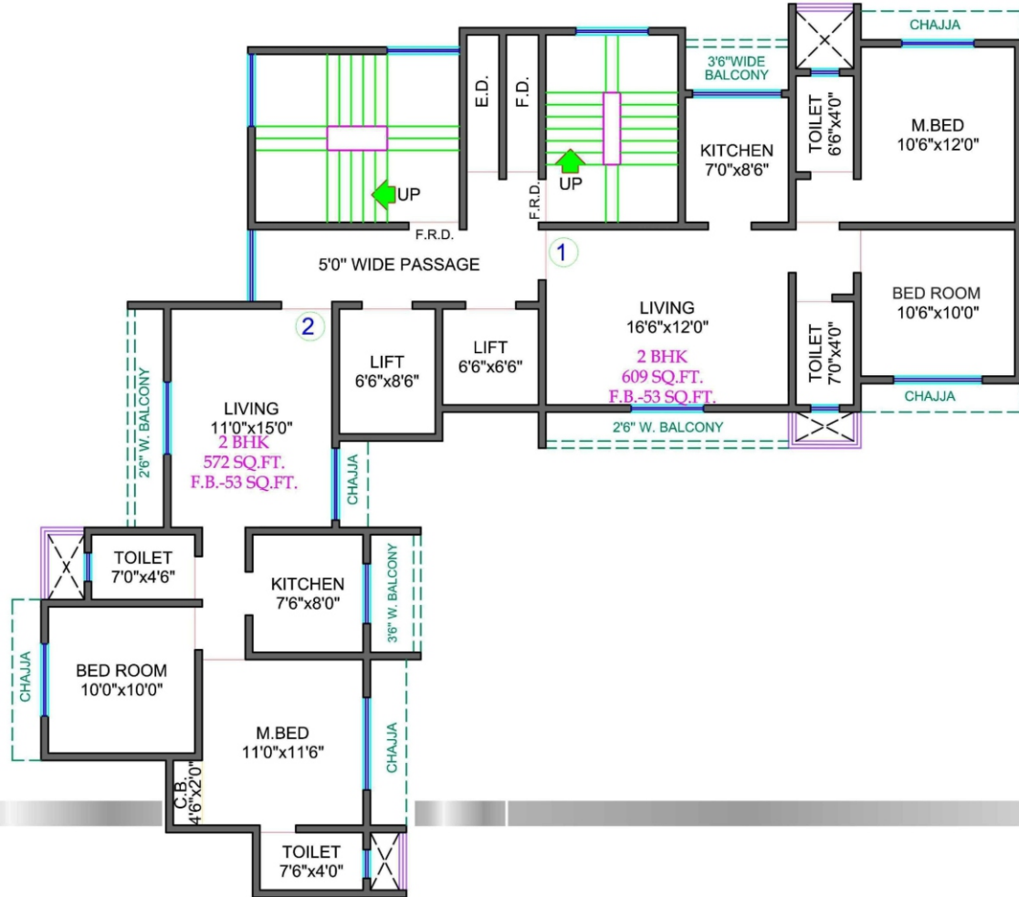
Typical Floor Plan B Wing
